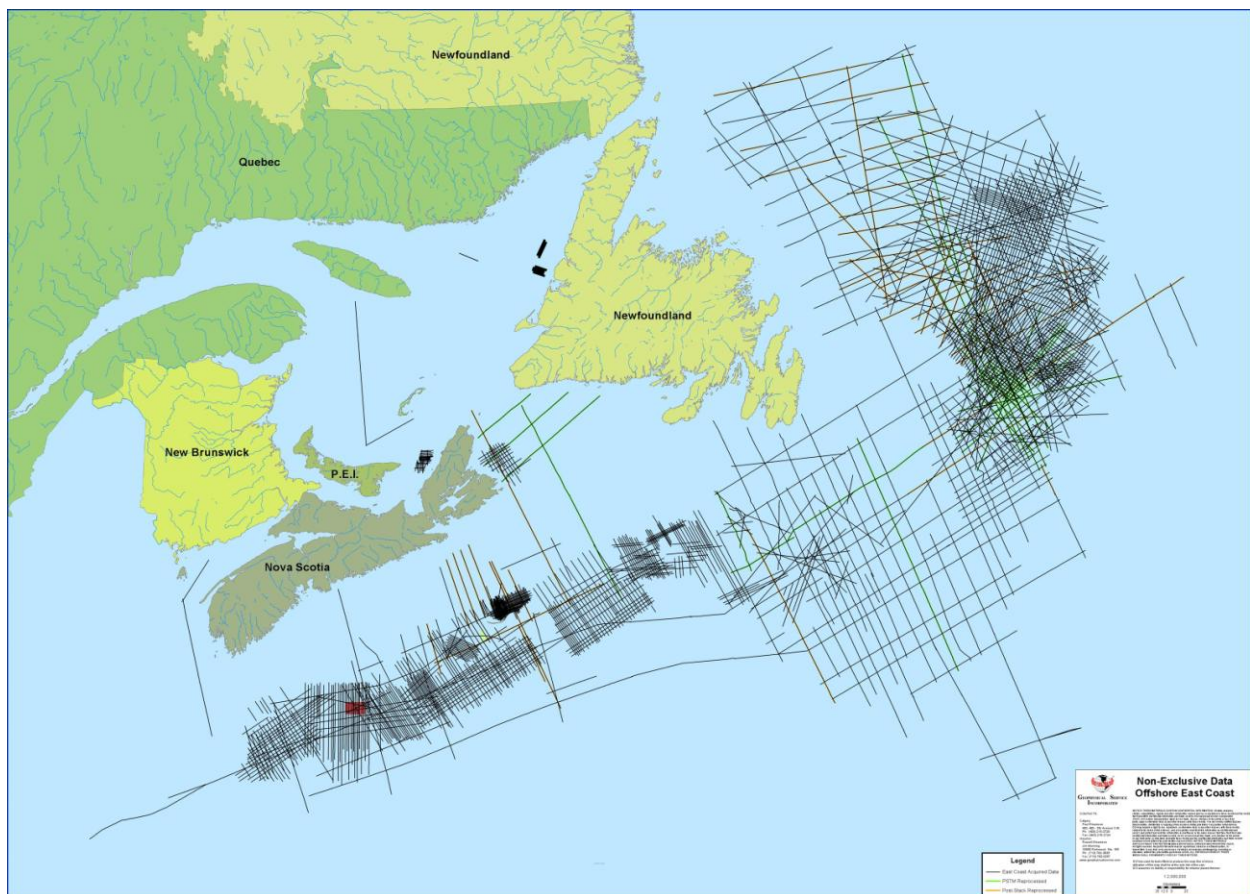
Figure 1. Example of non-exclusive (multi-client or spec) seismic coverage: GSI database in offshore East Coast Canada, comprising historic and more recent data.
